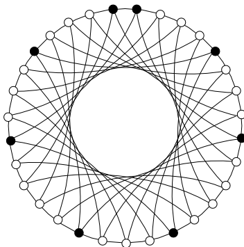
Figure 2: Facet of \{31,10\} -circulant: \sum_{v \in \circ} x_v + 2 \sum_{v \in \bullet} x_v \leq 4
