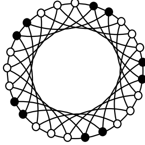
Figure 1: Facet of C^1 : \sum_{v \in \circ} x_v + 2 \sum_{v \in \bullet} x_v \leq 6
