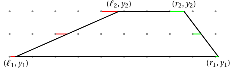
Figure 1: A quadrilateral for a pulse function p(x) defined by the arithmetic progression \{0.2, 0.45, 0.7\} with \varepsilon = 0.08 . The red line segments have length 0.28, 0.53 and 0.78 (bottom up) and the green line segments have length 0.12, 0.37 and 0.62 (bottom up). As the polygon is translated by x to the left, the number of integer points inside the polygon is 17 + p(x) .
