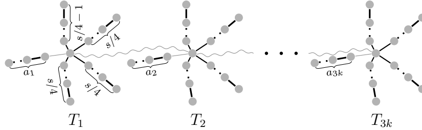
Figure 4: Construction for Theorem 4. Each gadget T_i is composed by an a_i -path connected to the root of an s -tree through an edge from A (straight grey). Each s -tree branches into four paths of (almost) the same length. Two adjacent gadgets in a path are connected through the roots of their s -trees with an edge from B (wiggled grey).
