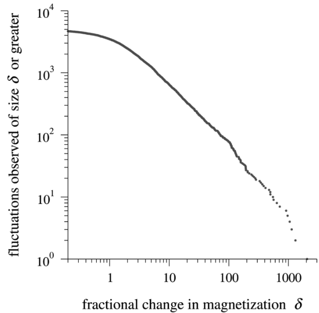
Figure 8. Cumulative histogram of the magnetization fluctuations of a 128 \times 128 nearest-neighbour Ising model on a square lattice. The model was simulated at a temperature of 2.5 times the spin–spin coupling for 100000 time steps using the cluster algorithm of Swendsen and Wang [46] and the magnetization per spin measured at intervals of ten steps. The fluctuations were calculated as the ratio \delta_i = 2(m_{i+1} - m_i)/(m_{i+1} + m_i) .
